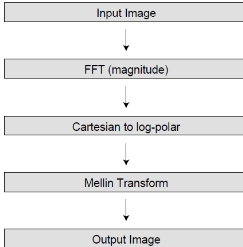
Figure 4.5. The Fourier-Mellin Transform.
