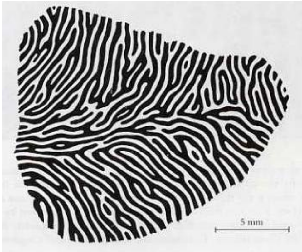
From macaque data
