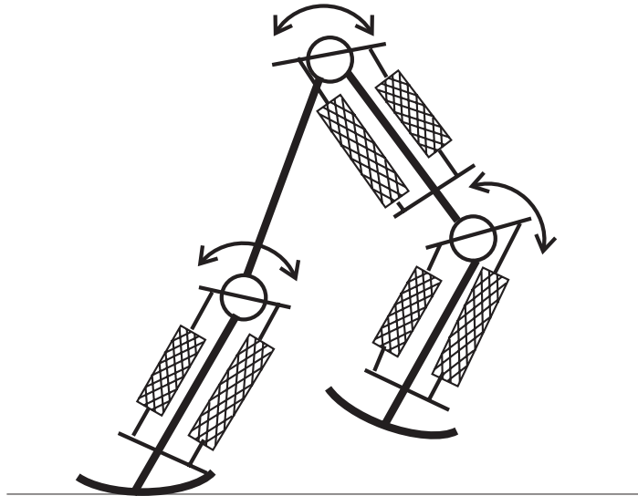
Fig. 2. A brief picture of the developed robot. It has three joints : two knees and one hip, and each joint is rotated by two muscles which are arranged by antagonistic pair like human ones.
