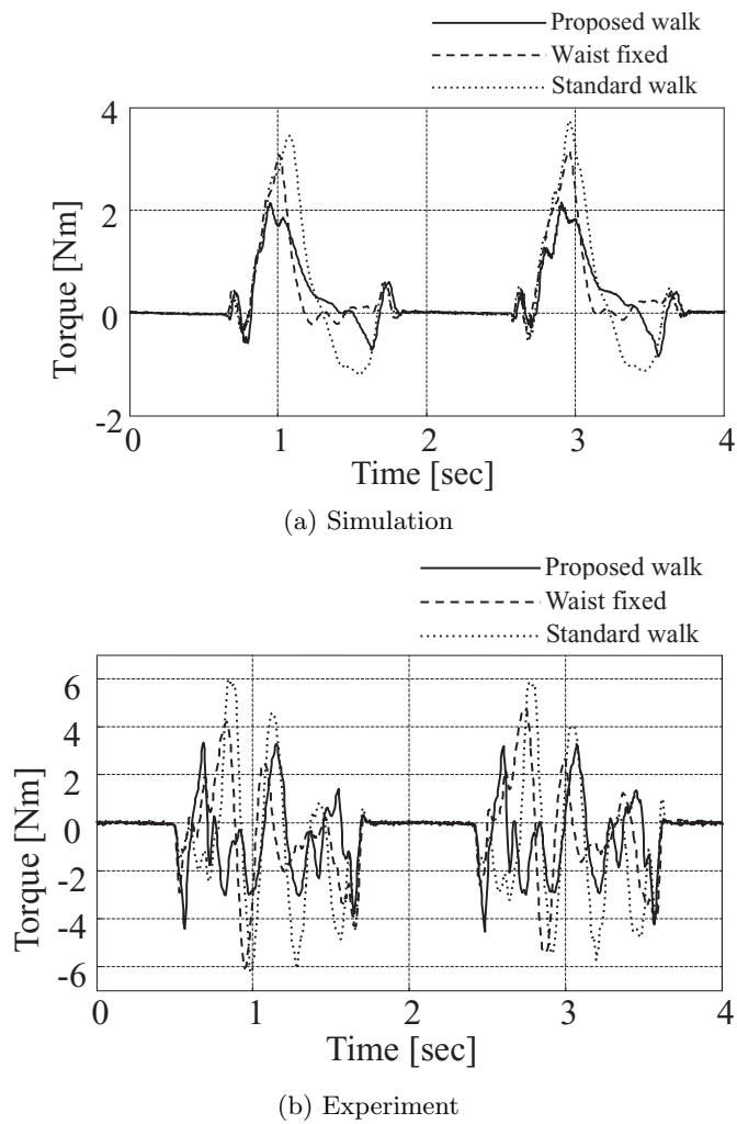
Fig. 16. Yaw-axis Torque of Stance Foot (0.83km/h)
