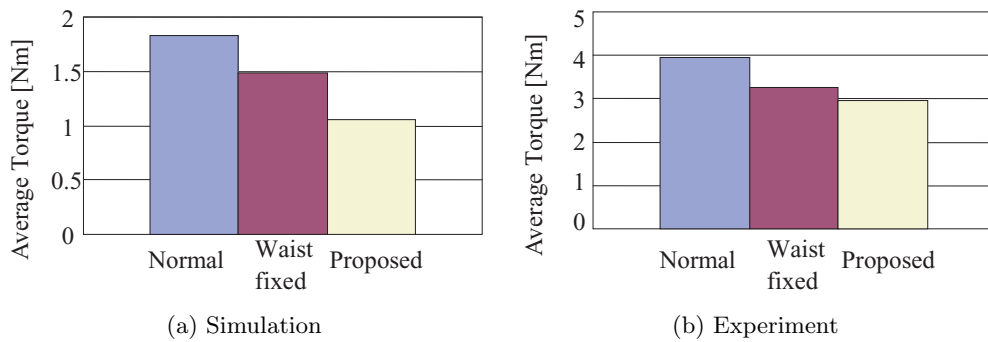
Fig. 17. Comparison of Average Torque (0.83km/h)
