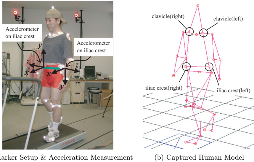
Fig. 1. 3-D Motion Capture
