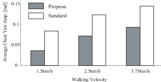
Fig. 19. Upper Body Rotation during Fast Walk (Average Yaw Amplitude)
