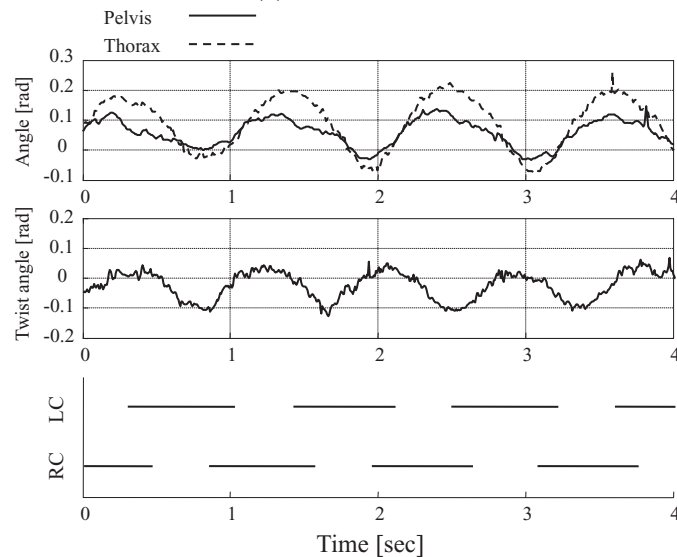
(b) Trunk-twistless Walk
