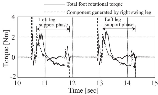
Fig. 12. Component of Stance Foot Torque (Simulation, 0.83km/h)
