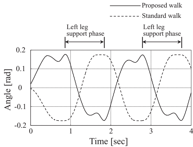
Fig. 14. Rotation Angle of Waist (Simulation, 0.83km/h)
