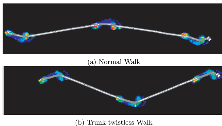
Fig. 7. Trajectory of COP
