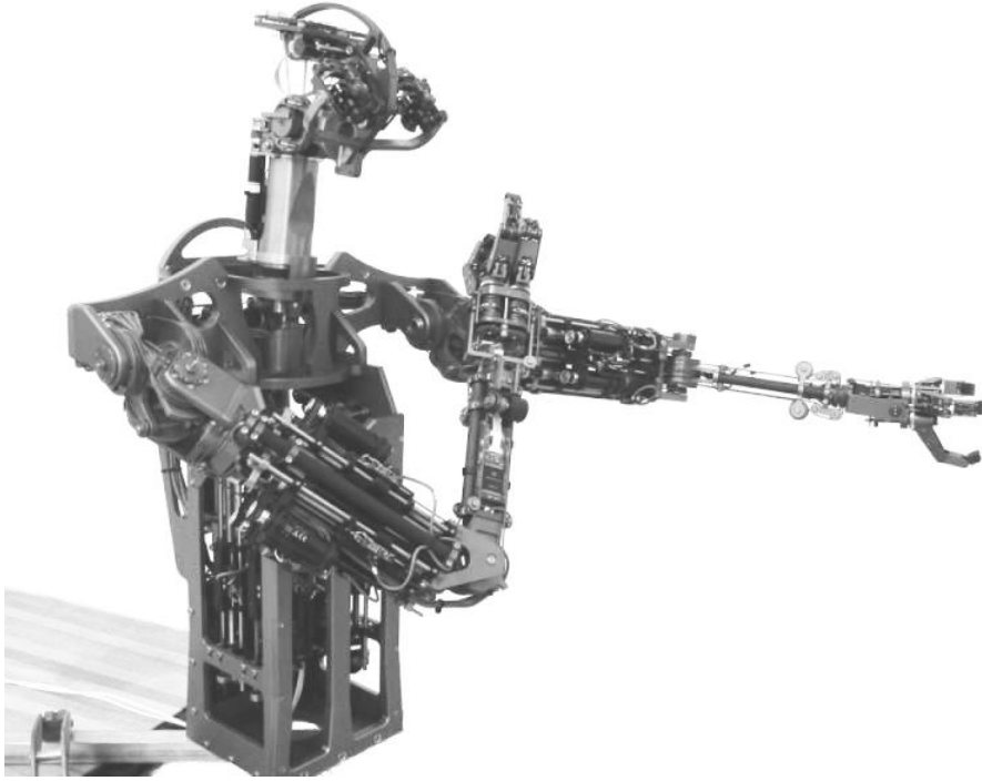
Fig. 1. The humanoid robot, Domo, under development. The robot has 29 DOF: six in each arm, four in each hand, two in the neck, and seven in the active vision head.
