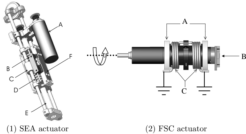
Fig. 4. (1) Model of the cable-drive SEA actuator. A brushless DC motor (A) imparts a linear motion to the inner drive carriage (C) through a precision ballscrew (E). The inner drive carriage transmits motion to the outer drive carriage (F) through two precompressed die springs (D). The deflection of the springs is measured with a linear potentiometer (B). (2) A simplified view of the FSC actuator. Two bearings (A) support the motor. The motor is attached to an external frame (ground) through two torsion springs (C). As the motor exerts a torque on a load, a deflection of the springs is created. This deflection is read by the torque sensing potentiometer (B).
