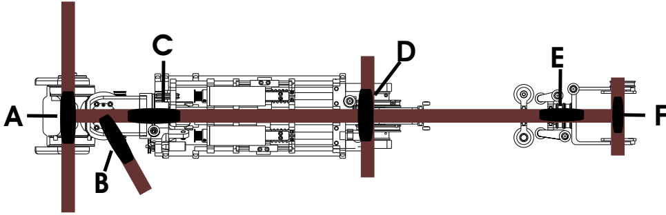
Fig. 6. The kinematic structure of Domo's arms. A compact cable-drive differential at the shoulder provides pitch (A) and roll (B). These two DOF are driven by actuators placed in the robot torso. The bicep of the arm contains four other actuators: shoulder yaw (C), elbow pitch (D), and wrist roll (E) and pitch (F) driven by two cables routed through the elbow.
