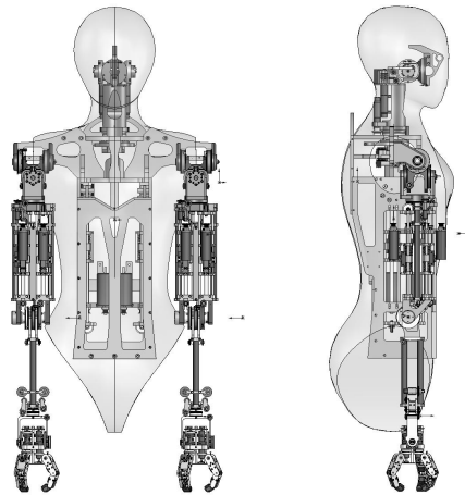
Fig. 2. Drawing of Domo overlaid with a human silhouette. The proportions of the robot were chosen to be non-intimidating during human-robot interactions.
