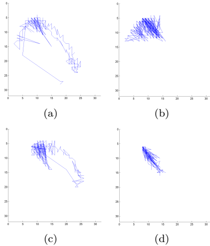
Figure 3: Experiment number 1. Learning to move a colored object from the upper left corner of the visual field to the center of it. Position of the center of the object in the visual field during the learning cycles in the interval (a) [1, 400]. (b) [401, 800]. (c) [801, 1200]. (d) [1201, 1602].
