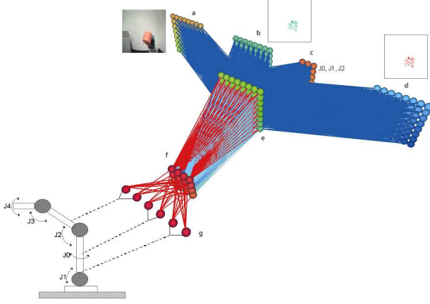
Figure 1: Neural structure and its connections to the robot’s sensors and motors. Neuronal areas: (a) RedColorField. (b) RedMovementToRightField. (c) ProprioceptiveField. (d) RedMovementToLeftField. (e) NeuronalField. (f) MotorField. (g) MotorActivites.
