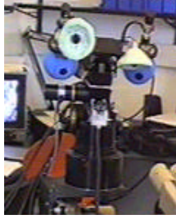
Figure 1: The experimental setup. Right: the robot system is a 5 DOF binocular head integrating an artificial vestibular system (i.e. the white bloc in the centre of the picture). Left: a block diagram of the NN, its inputs (optic flow, head velocity) and output (eye velocity).
